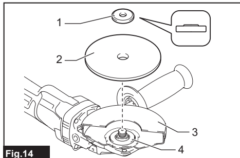
► 1. Lock nut 2. Abrasive cut-off wheel 3. Wheel guard for abrasive cut-off wheel 4. Inner flange
